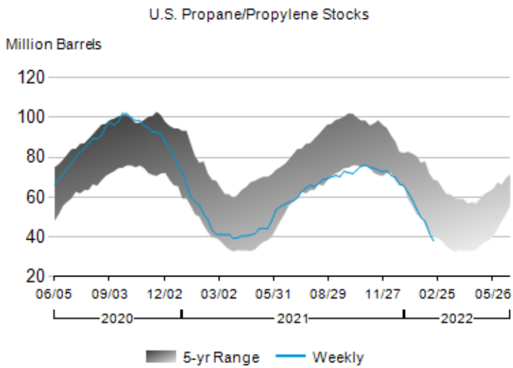
Figure 6. Stocks of Propane/Propylene by PAD District, June 2020 to Present
