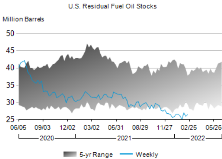
Figure 5. Stocks of Residual Fuel Oil by PAD District, June 2020 to Present
